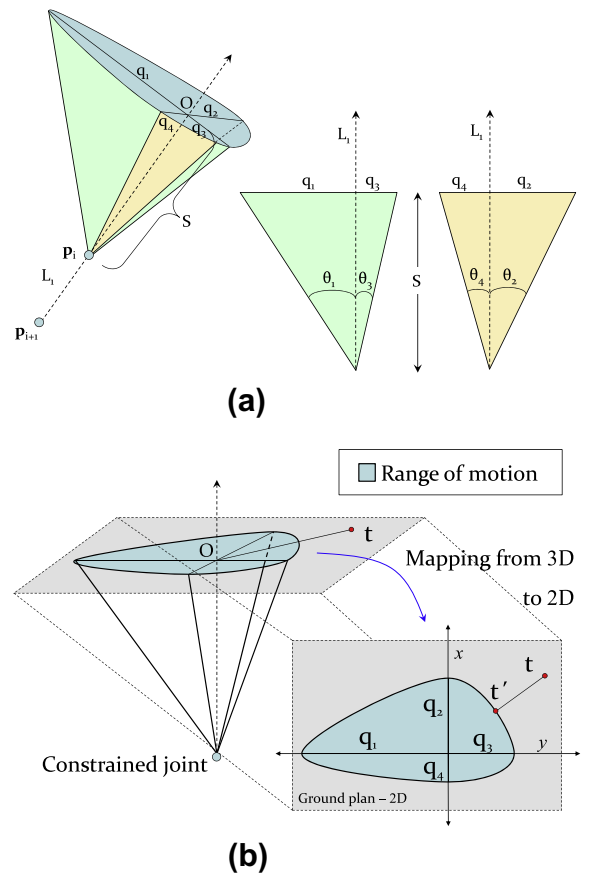
Fig. 4. (a) The ball-and-socket joint, p_i , with its associated irregular cone which defines the allowed range of motion. (b) Shows the composite ellipsoidal shape created by the distances q_j mapped from 3D to 2D.
